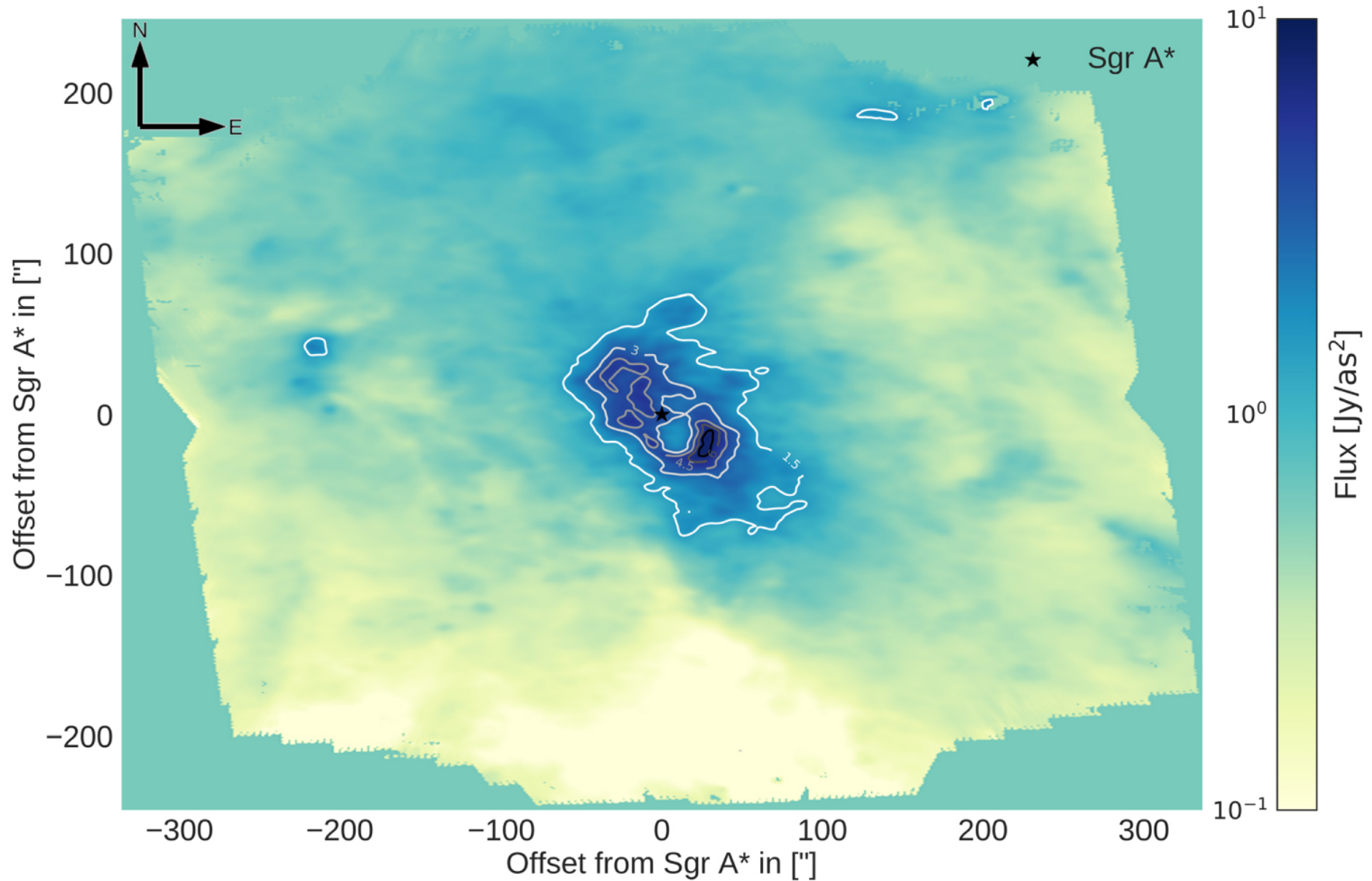
Figure 9. from A Detection of Sgr A* in the Far Infrared null 2018 APJ 862 129 doi:10.3847/1538-4357/aacd4b https://dx.doi.org/10.3847/1538-4357/aacd4b © 2018. The American Astronomical Society. All rights reserved.
