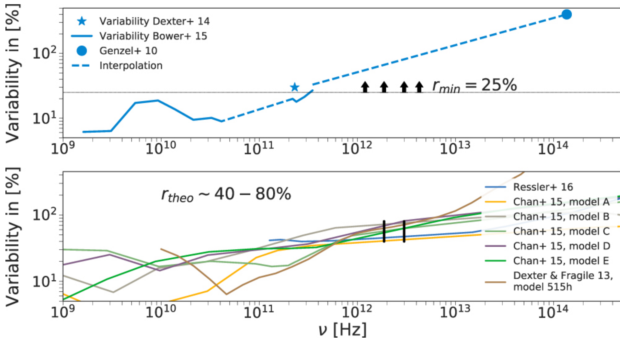
Figure 6. from A Detection of Sgr A* in the Far Infrared null 2018 APJ 862 129 doi:10.3847/1538-4357/aacd4b https://dx.doi.org/10.3847/1538-4357/aacd4b © 2018. The American Astronomical Society. All rights reserved.
