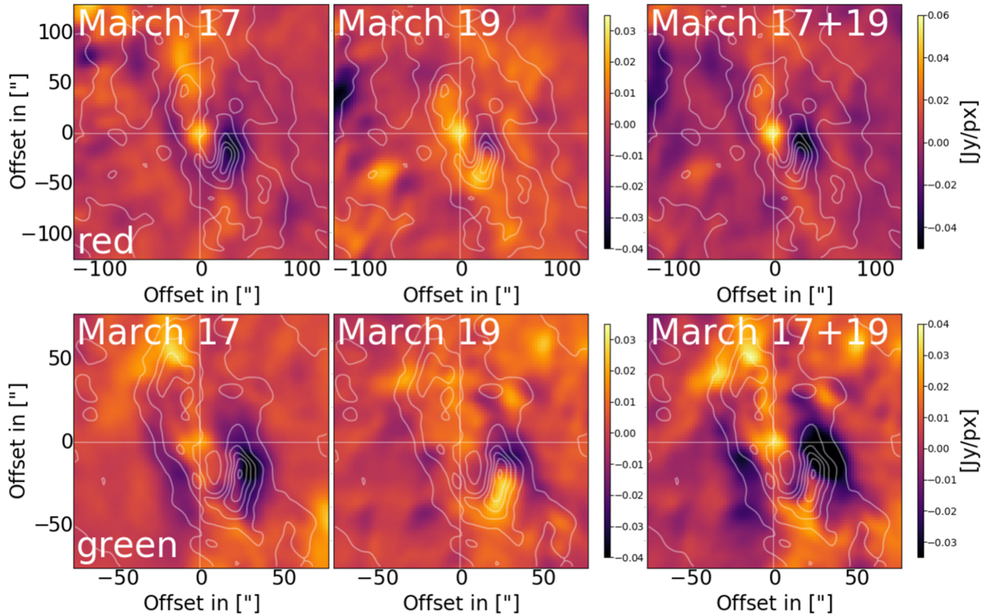
Figure 5. from A Detection of Sgr A* in the Far Infrared null 2018 APJ 862 129 doi:10.3847/1538-4357/aacd4b https://dx.doi.org/10.3847/1538-4357/aacd4b © 2018. The American Astronomical Society. All rights reserved.
