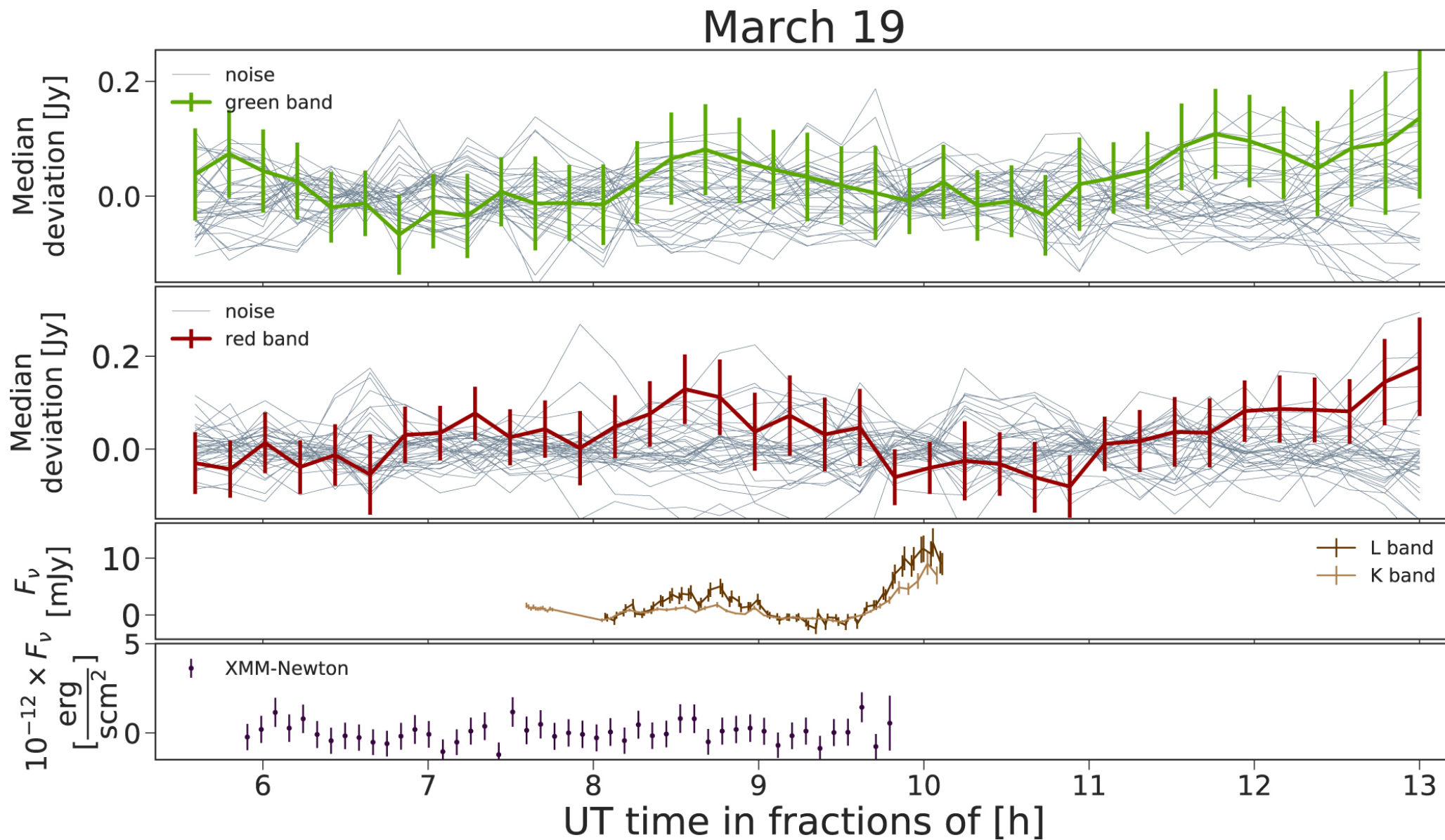
Figure 4. from A Detection of Sgr A* in the Far Infrared null 2018 APJ 862 129 doi:10.3847/1538-4357/aacd4b https://dx.doi.org/10.3847/1538-4357/aacd4b © 2018. The American Astronomical Society. All rights reserved.
