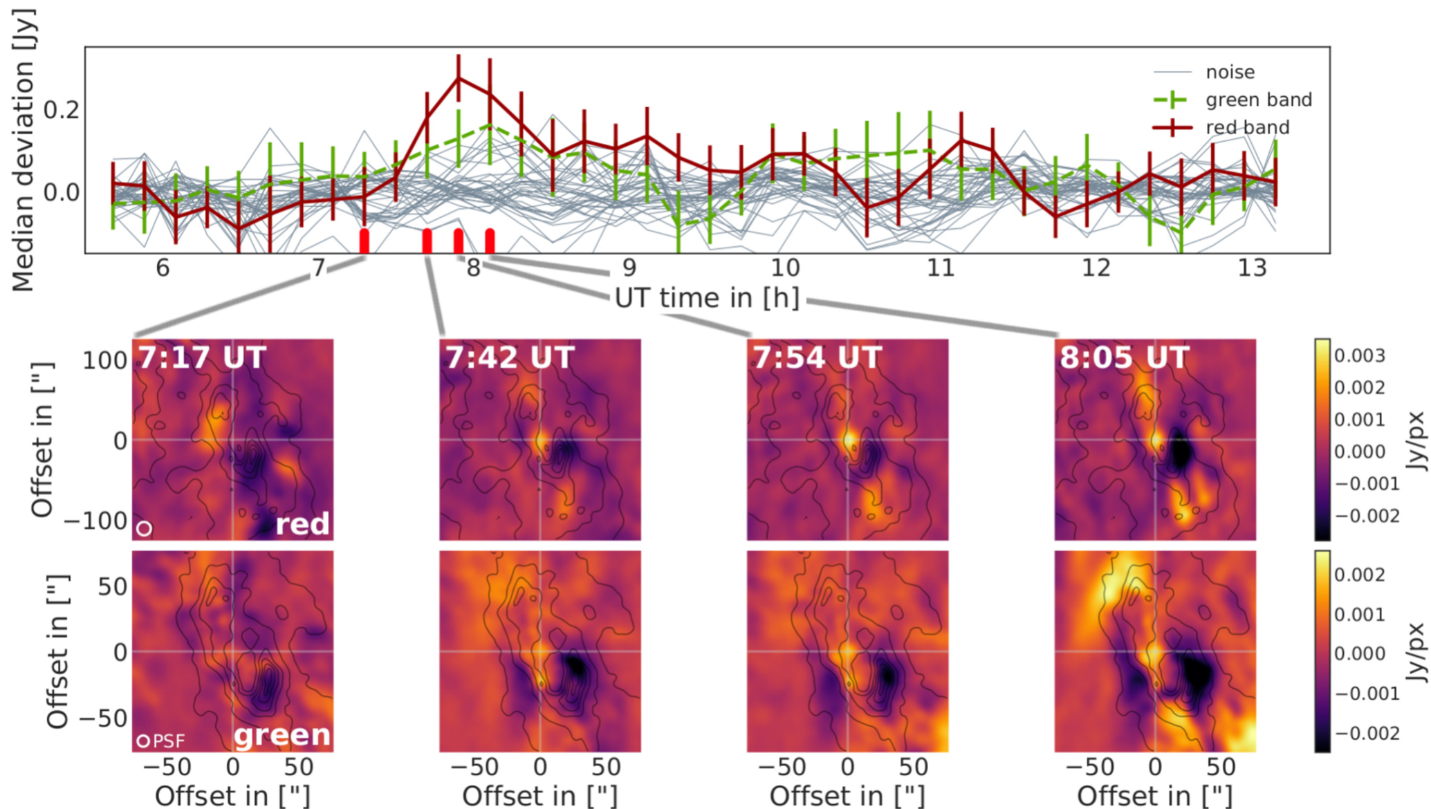
Figure 2. from A Detection of Sgr A* in the Far Infrared null 2018 APJ 862 129 doi:10.3847/1538-4357/aacd4b https://dx.doi.org/10.3847/1538-4357/aacd4b © 2018. The American Astronomical Society. All rights reserved.
