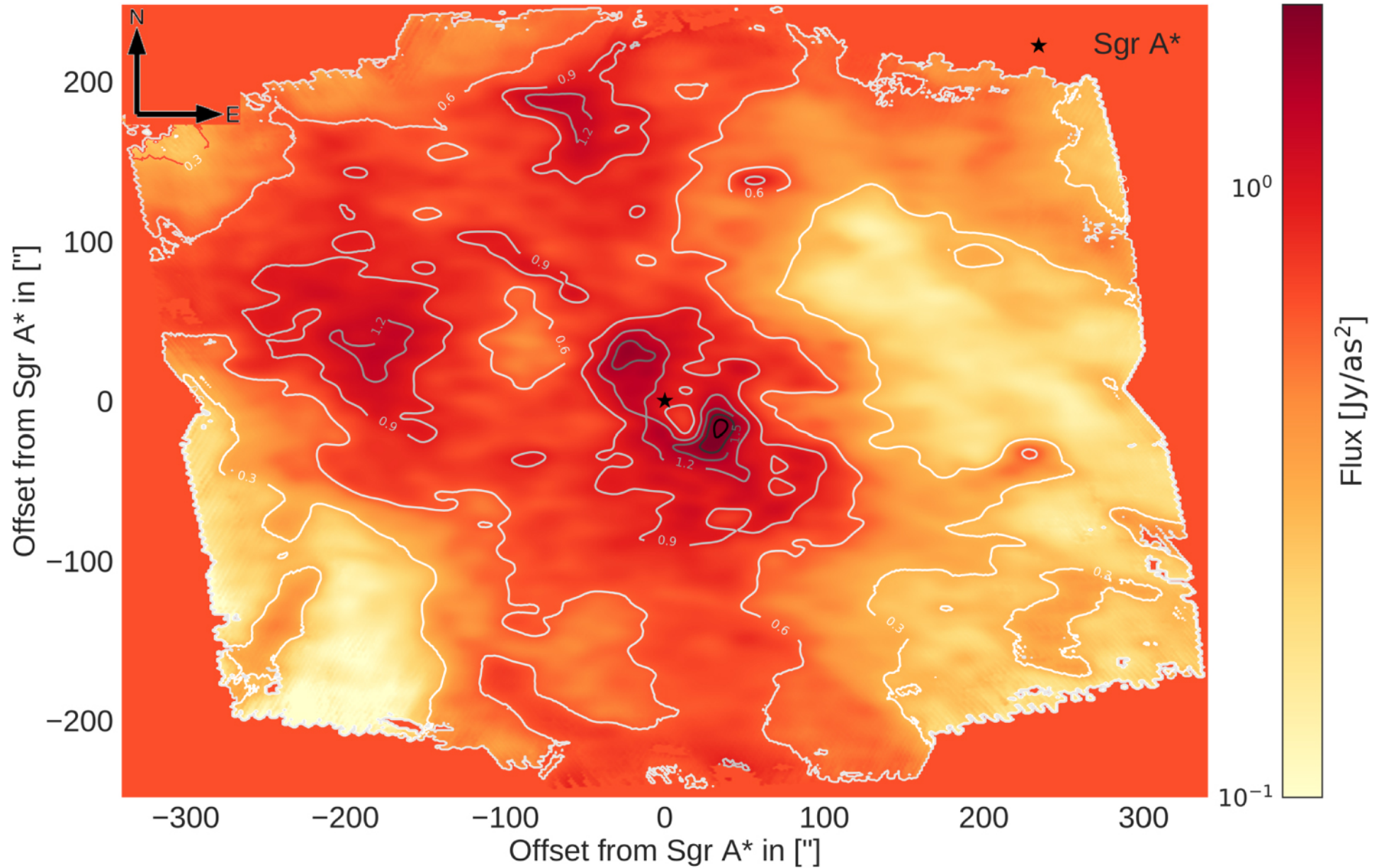
Figure 11. from A Detection of Sgr A* in the Far Infrared null 2018 APJ 862 129 doi:10.3847/1538-4357/aacd4b https://dx.doi.org/10.3847/1538-4357/aacd4b © 2018. The American Astronomical Society. All rights reserved.
