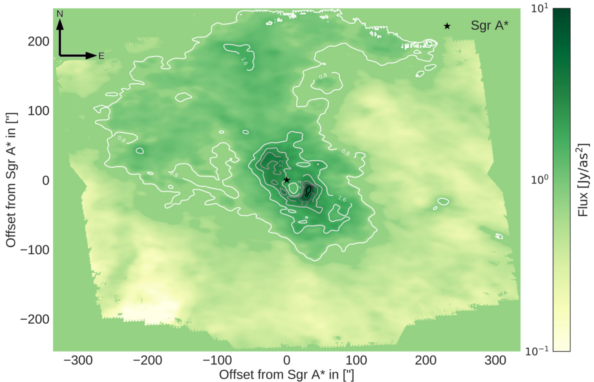
Figure 10. from A Detection of Sgr A* in the Far Infrared null 2018 APJ 862 129 doi:10.3847/1538-4357/aacd4b https://dx.doi.org/10.3847/1538-4357/aacd4b © 2018. The American Astronomical Society. All rights reserved.
