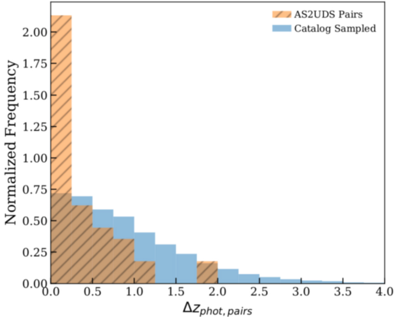
Figure 4. from An ALMA Survey of the SCUBA-2 Cosmology Legacy Survey UKIDSS/UDS Field: Number Counts of Submillimeter Galaxies null 2018 APJ 860 161 doi:10.3847/1538-4357/aac5e5 https://dx.doi.org/10.3847/1538-4357/aac5e5 © 2018. The American Astronomical Society. All rights reserved.
