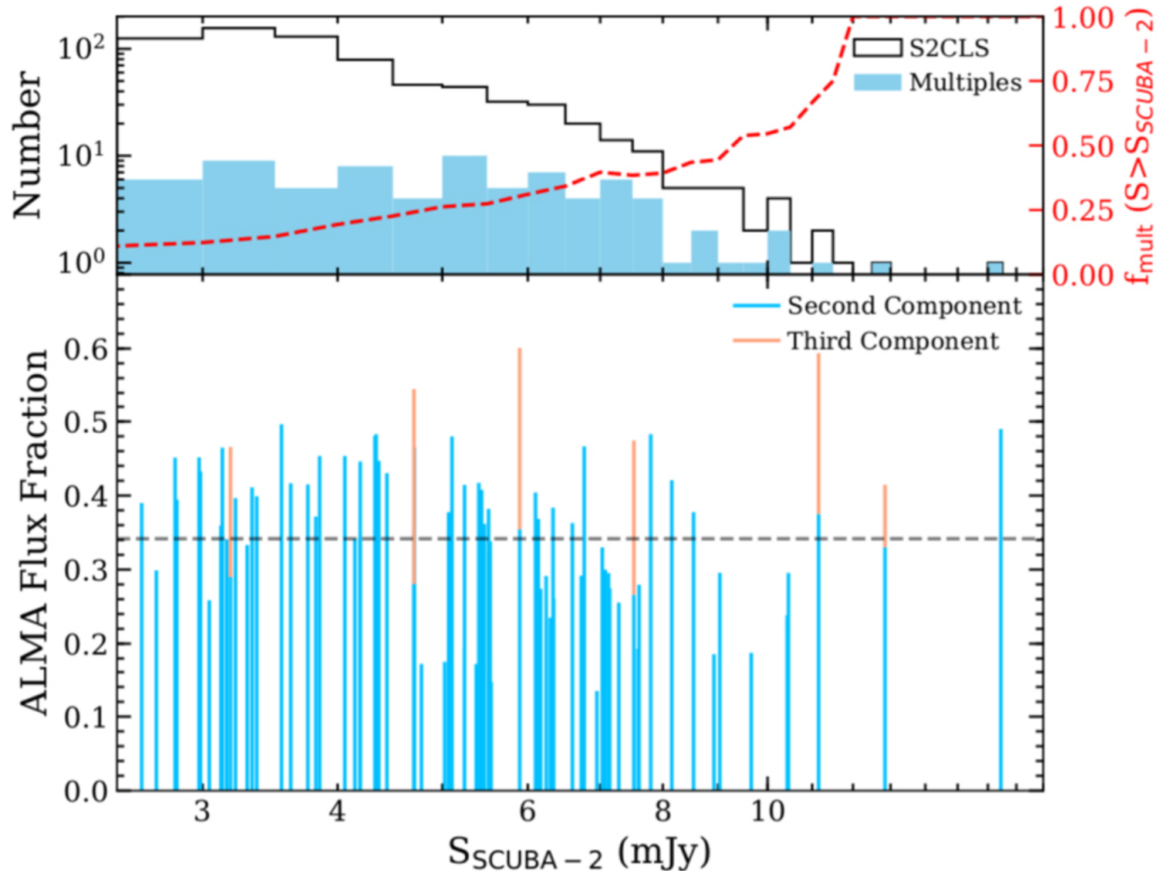
Figure 3. from An ALMA Survey of the SCUBA-2 Cosmology Legacy Survey UKIDSS/UDS Field: Number Counts of Submillimeter Galaxies null 2018 APJ 860 161 doi:10.3847/1538-4357/aac5e5 https://dx.doi.org/10.3847/1538-4357/aac5e5 © 2018. The American Astronomical Society. All rights reserved.
