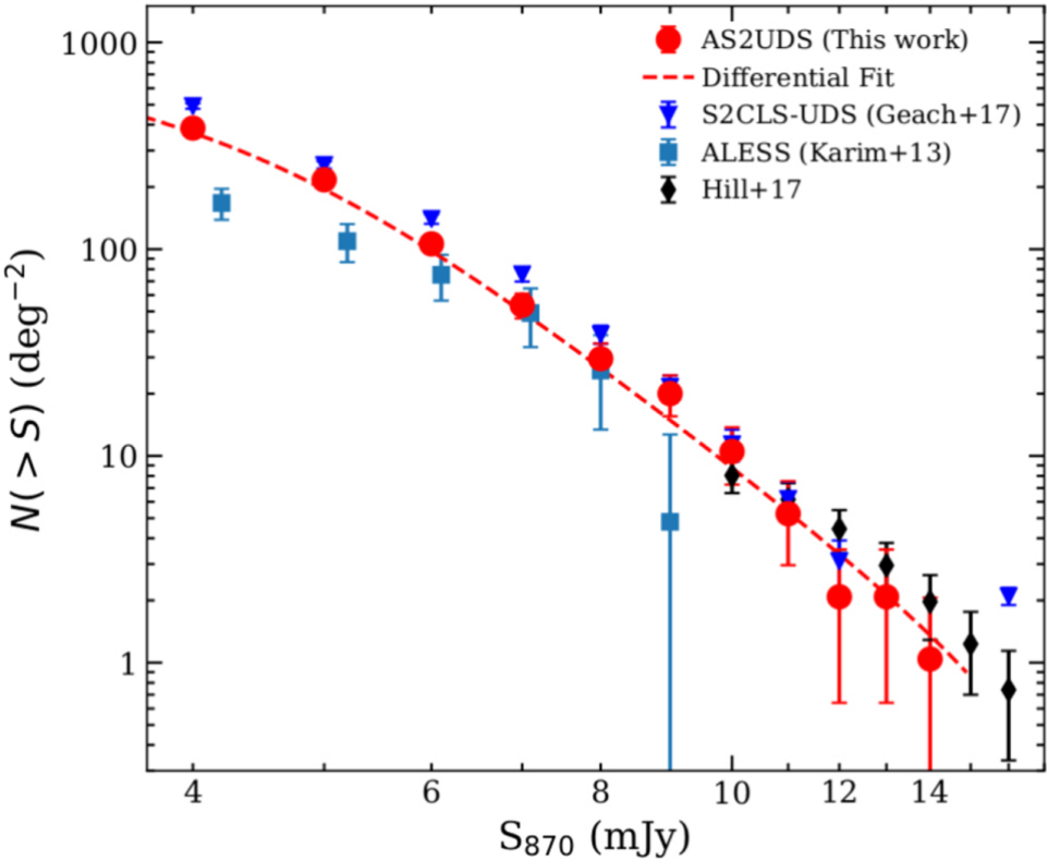
Figure 2. from An ALMA Survey of the SCUBA-2 Cosmology Legacy Survey UKIDSS/UDS Field: Number Counts of Submillimeter Galaxies null 2018 APJ 860 161 doi:10.3847/1538-4357/aac5e5 https://dx.doi.org/10.3847/1538-4357/aac5e5 © 2018. The American Astronomical Society. All rights reserved.
