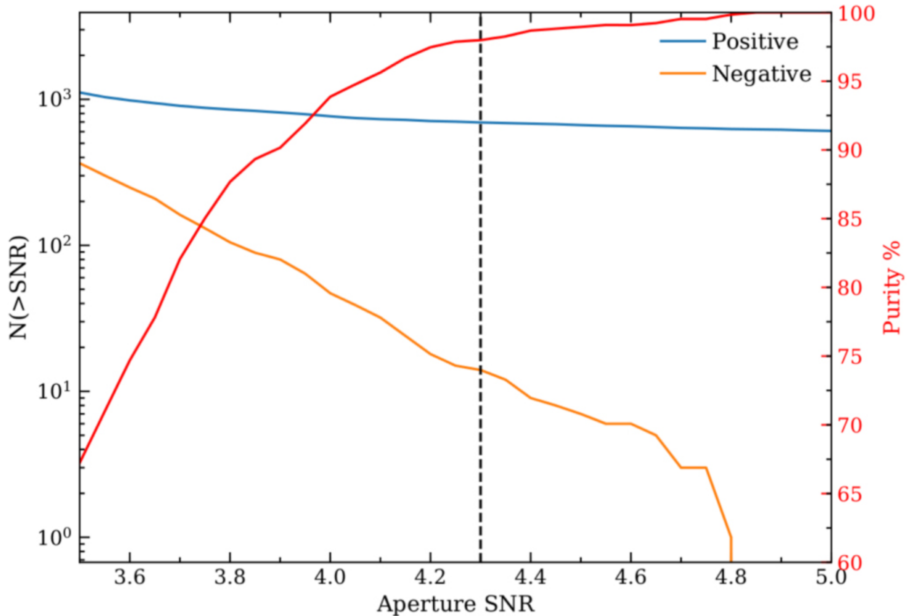
Figure 1. from An ALMA Survey of the SCUBA-2 Cosmology Legacy Survey UKIDSS/UDS Field: Number Counts of Submillimeter Galaxies null 2018 APJ 860 161 doi:10.3847/1538-4357/aac5e5 https://dx.doi.org/10.3847/1538-4357/aac5e5 © 2018. The American Astronomical Society. All rights reserved.
