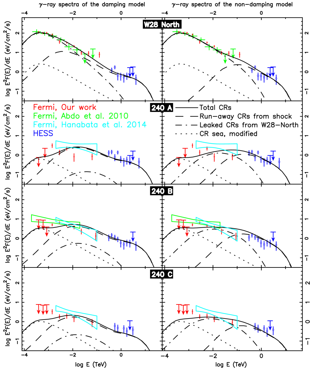
Figure 9. from Leaked GeV CRs from a Broken Shell: Explaining 9 Years of Fermi-LAT Data of SNR W28 null 2018 APJ 860 69 doi:10.3847/1538-4357/aac37b https://dx.doi.org/10.3847/1538-4357/aac37b © 2018. The American Astronomical Society. All rights reserved.
