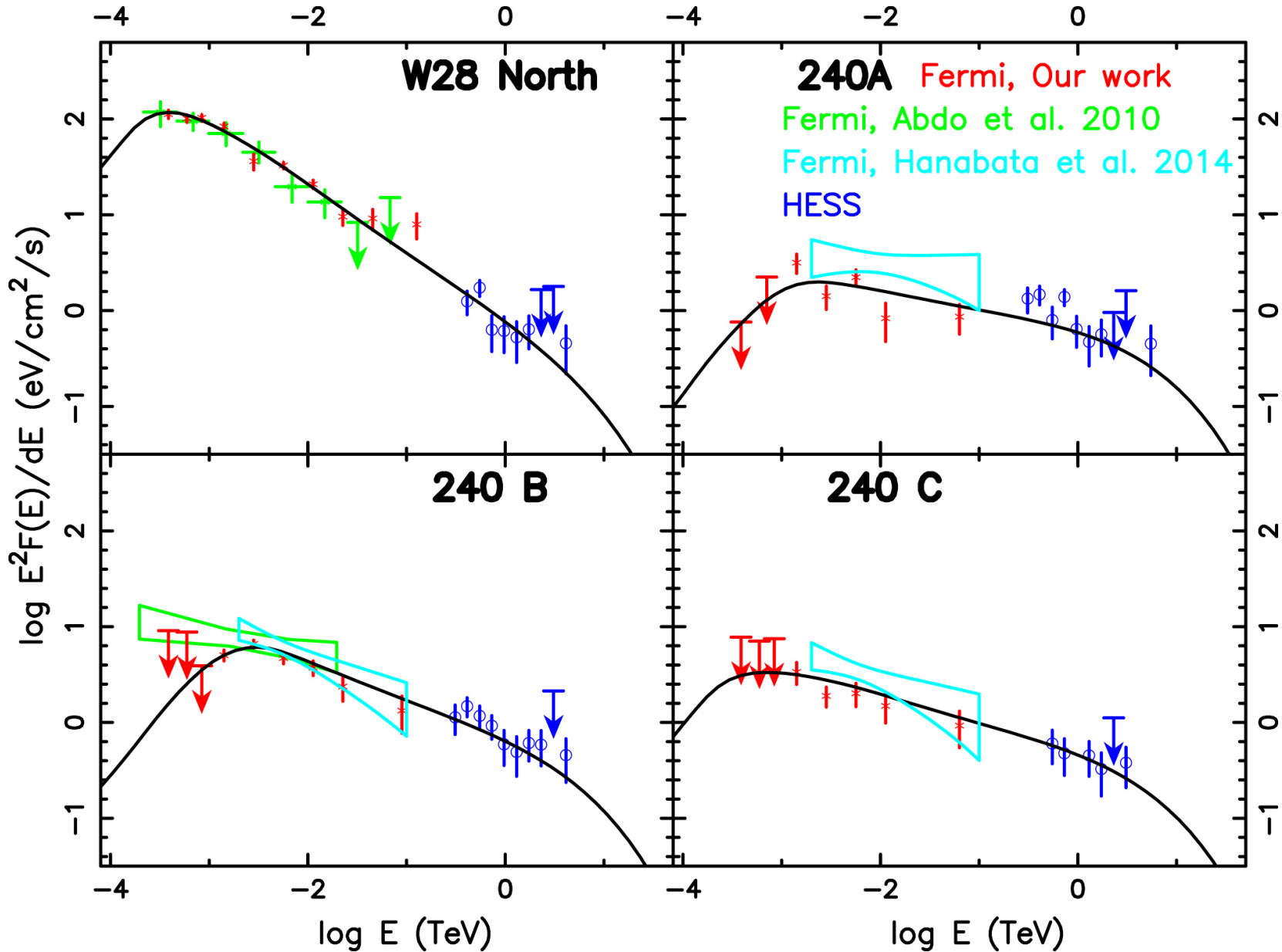
Figure 6. from Leaked GeV CRs from a Broken Shell: Explaining 9 Years of Fermi-LAT Data of SNR W28 null 2018 APJ 860 69 doi:10.3847/1538-4357/aac37b https://dx.doi.org/10.3847/1538-4357/aac37b © 2018. The American Astronomical Society. All rights reserved.
