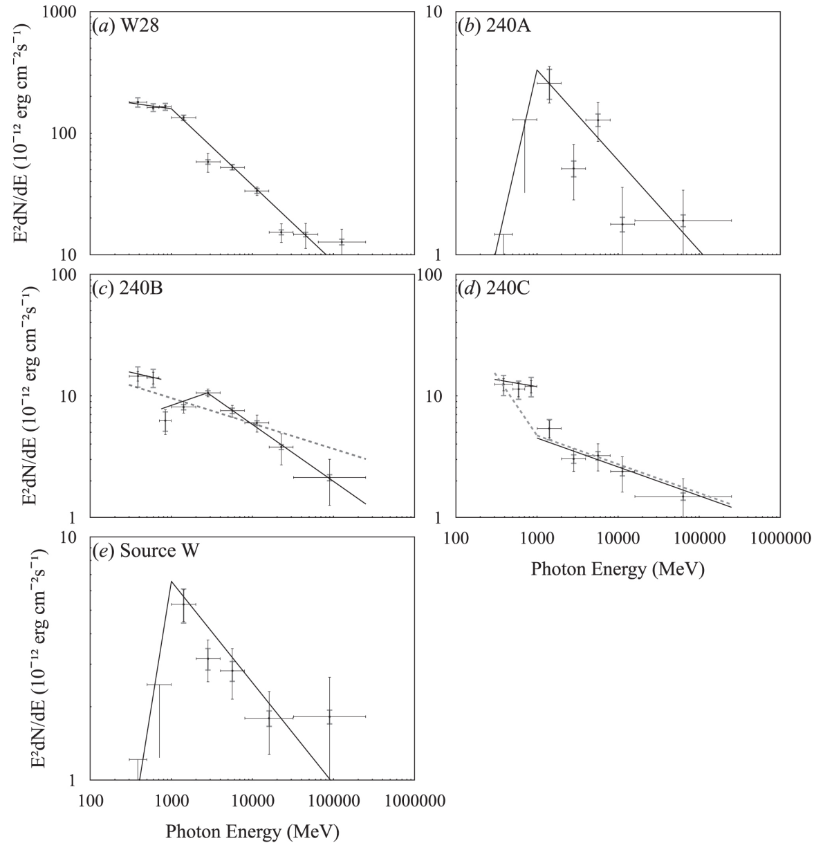
Figure 5. from Leaked GeV CRs from a Broken Shell: Explaining 9 Years of Fermi-LAT Data of SNR W28 null 2018 APJ 860 69 doi:10.3847/1538-4357/aac37b https://dx.doi.org/10.3847/1538-4357/aac37b © 2018. The American Astronomical Society. All rights reserved.
