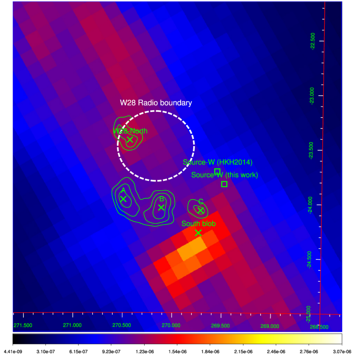
Figure 4. from Leaked GeV CRs from a Broken Shell: Explaining 9 Years of Fermi-LAT Data of SNR W28 null 2018 APJ 860 69 doi:10.3847/1538-4357/aac37b https://dx.doi.org/10.3847/1538-4357/aac37b © 2018. The American Astronomical Society. All rights reserved.
