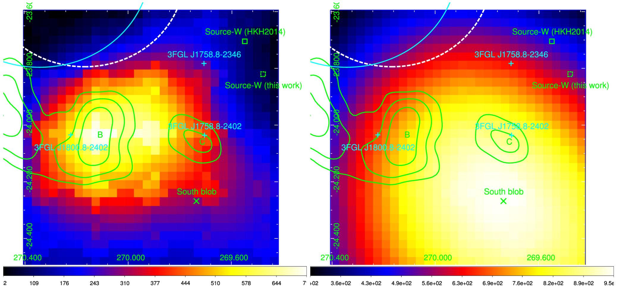
Figure 3. from Leaked GeV CRs from a Broken Shell: Explaining 9 Years of Fermi-LAT Data of SNR W28 null 2018 APJ 860 69 doi:10.3847/1538-4357/aac37b https://dx.doi.org/10.3847/1538-4357/aac37b © 2018. The American Astronomical Society. All rights reserved.
