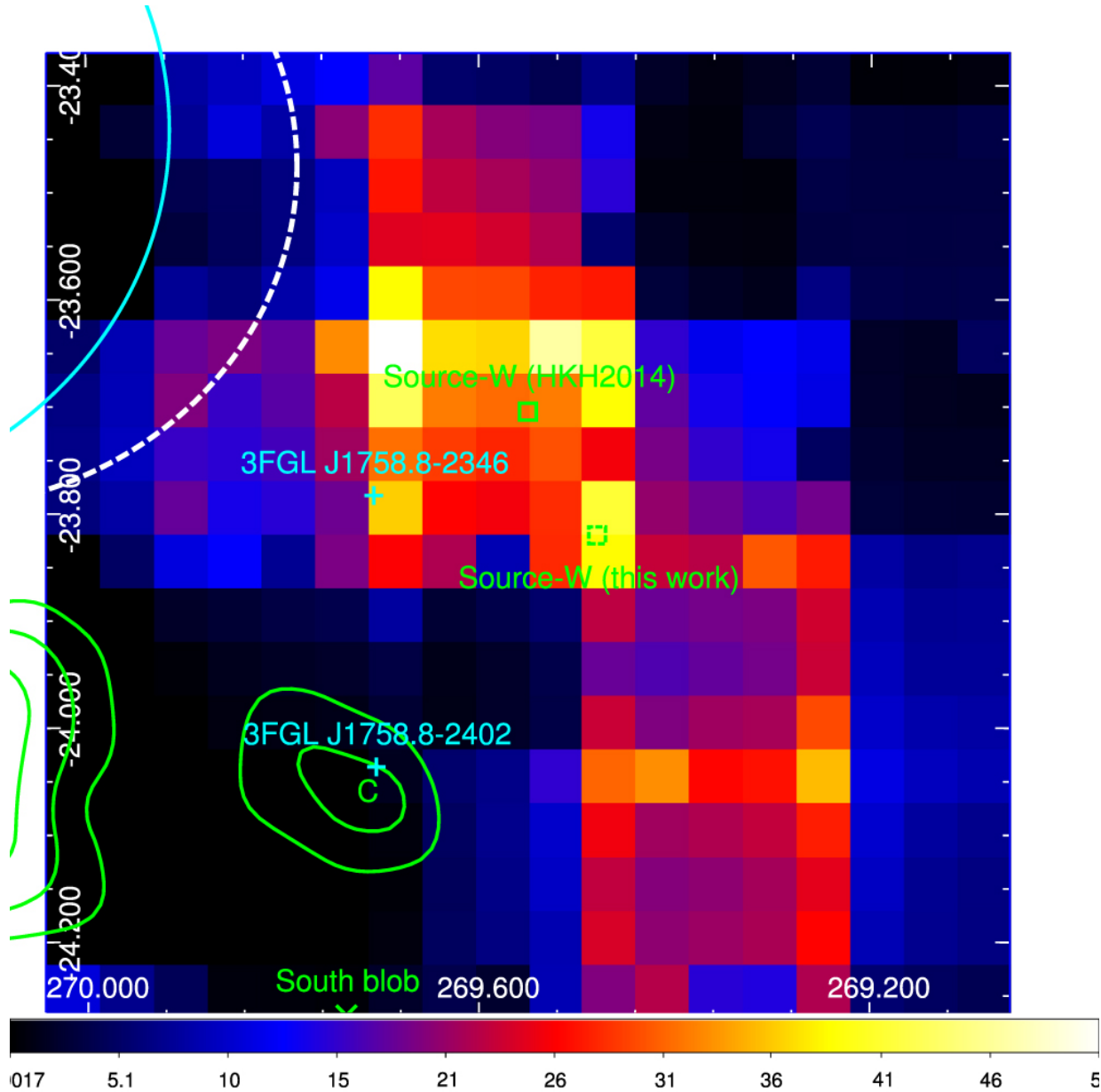
Figure 2. from Leaked GeV CRs from a Broken Shell: Explaining 9 Years of Fermi-LAT Data of SNR W28 null 2018 APJ 860 69 doi:10.3847/1538-4357/aac37b https://dx.doi.org/10.3847/1538-4357/aac37b © 2018. The American Astronomical Society. All rights reserved.
