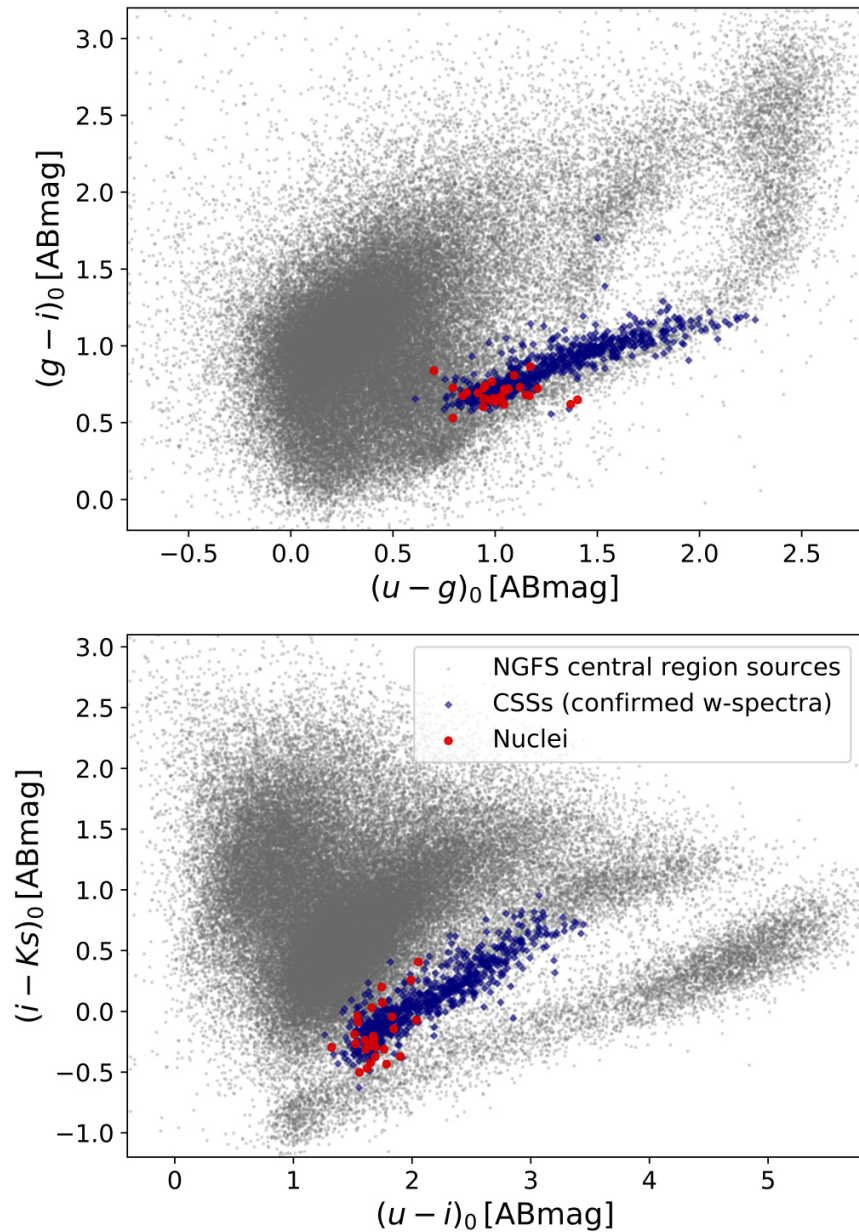
Figure 6. from The Next Generation Fornax Survey (NGFS). IV. Mass and Age Bimodality of Nuclear Clusters in the Fornax Core Region null 2018 APJ 860 4 doi:10.3847/1538-4357/aac1b8 https://dx.doi.org/10.3847/1538-4357/aac1b8 © 2018. The American Astronomical Society. All rights reserved.
