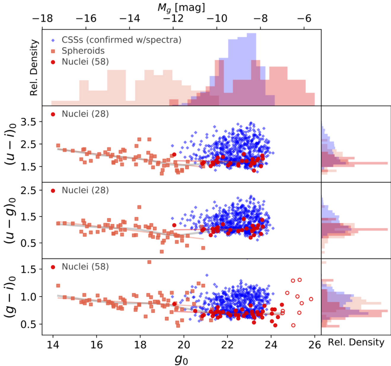
Figure 5. from The Next Generation Fornax Survey (NGFS). IV. Mass and Age Bimodality of Nuclear Clusters in the Fornax Core Region null 2018 APJ 860 4 doi:10.3847/1538-4357/aac1b8 https://dx.doi.org/10.3847/1538-4357/aac1b8 © 2018. The American Astronomical Society. All rights reserved.
