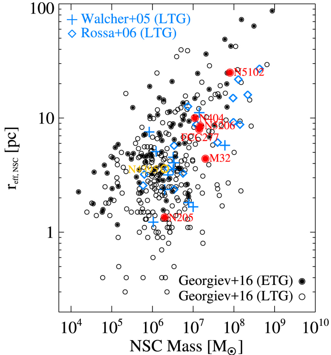
Figure 9. from Nearby Early-type Galactic Nuclei at High Resolution: Dynamical Black Hole and Nuclear Star Cluster Mass Measurements null 2018 APJ 858 118 doi:10.3847/1538-4357/aabe28 https://dx.doi.org/10.3847/1538-4357/aabe28 © 2018. The American Astronomical Society. All rights reserved.
