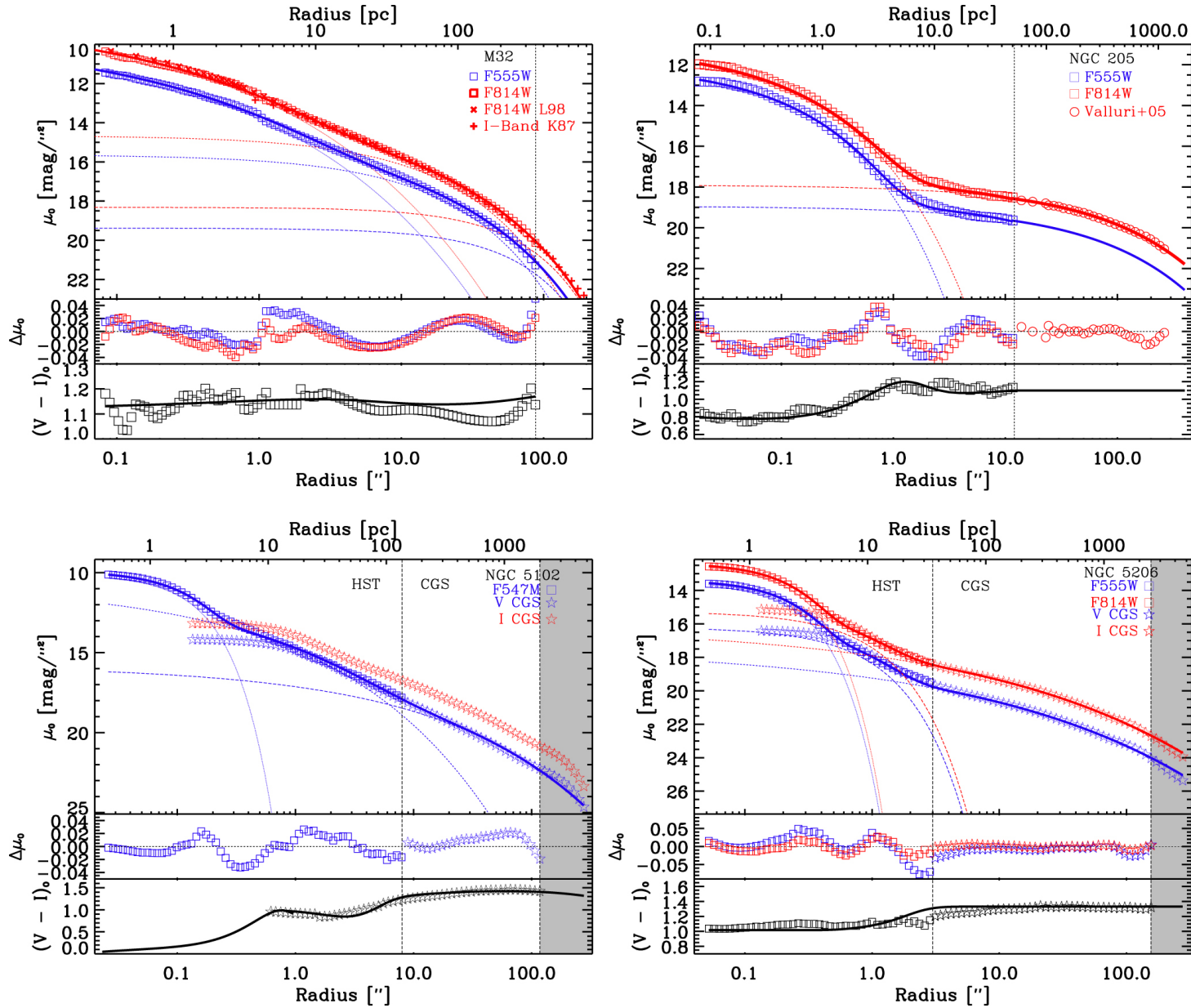
Figure 1. from Nearby Early-type Galactic Nuclei at High Resolution: Dynamical Black Hole and Nuclear Star Cluster Mass Measurements null 2018 APJ 858 118 doi:10.3847/1538-4357/aabe28 https://dx.doi.org/10.3847/1538-4357/aabe28 © 2018. The American Astronomical Society. All rights reserved.
