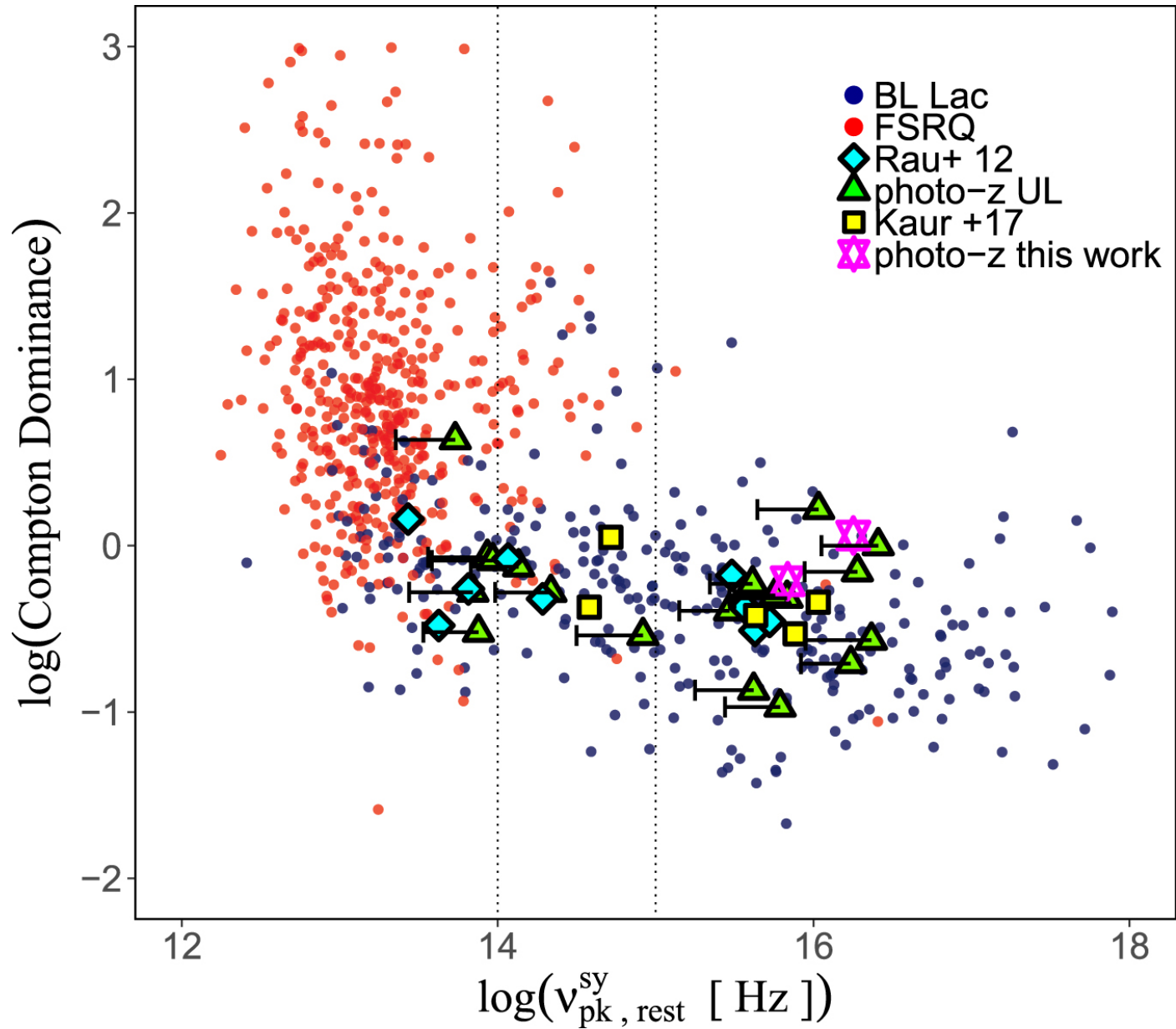
Figure 6. from New High-z BL Lacs Using the Photometric Method with Swift and SARA null 2018 APJ 859 80 doi:10.3847/1538-4357/aabdec https://dx.doi.org/10.3847/1538-4357/aabdec © 2018. The American Astronomical Society. All rights reserved.
