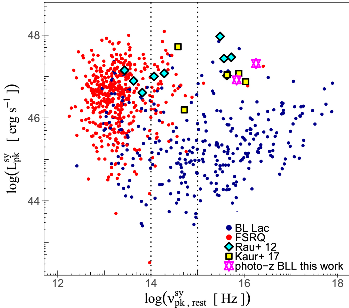
Figure 5. from New High-z BL Lacs Using the Photometric Method with Swift and SARA null 2018 APJ 859 80 doi:10.3847/1538-4357/aabdec https://dx.doi.org/10.3847/1538-4357/aabdec © 2018. The American Astronomical Society. All rights reserved.
