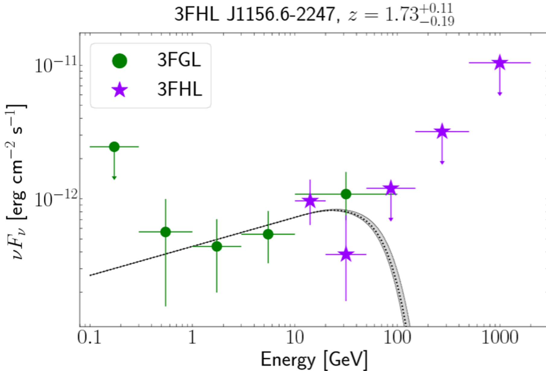
Figure 3. from New High-z BL Lacs Using the Photometric Method with Swift and SARA null 2018 APJ 859 80 doi:10.3847/1538-4357/aabdec https://dx.doi.org/10.3847/1538-4357/aabdec © 2018. The American Astronomical Society. All rights reserved.
