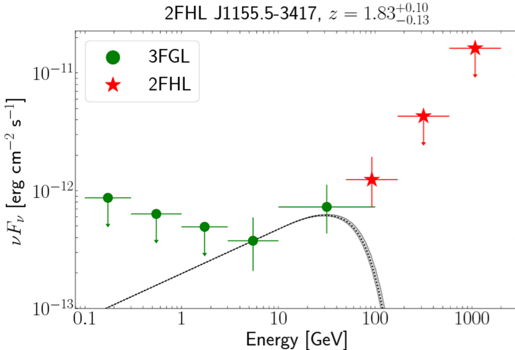
Figure 2. from New High-z BL Lacs Using the Photometric Method with Swift and SARA null 2018 APJ 859 80 doi:10.3847/1538-4357/aabdec https://dx.doi.org/10.3847/1538-4357/aabdec © 2018. The American Astronomical Society. All rights reserved.
