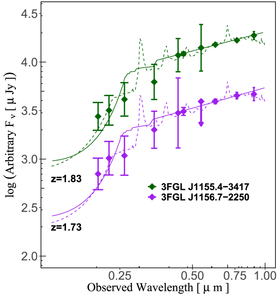
Figure 1. from New High-z BL Lacs Using the Photometric Method with Swift and SARA null 2018 APJ 859 80 doi:10.3847/1538-4357/aabdec https://dx.doi.org/10.3847/1538-4357/aabdec © 2018. The American Astronomical Society. All rights reserved.
