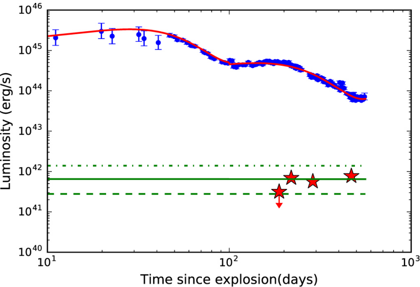
Figure 1. from Persistent X-Ray Emission from ASASSN-15lh: Massive Ejecta and Pre-SLSN Dense Wind? null 2018 APJ 859 123 doi:10.3847/1538-4357/aabcca https://dx.doi.org/10.3847/1538-4357/aabcca © 2018. The American Astronomical Society. All rights reserved.
