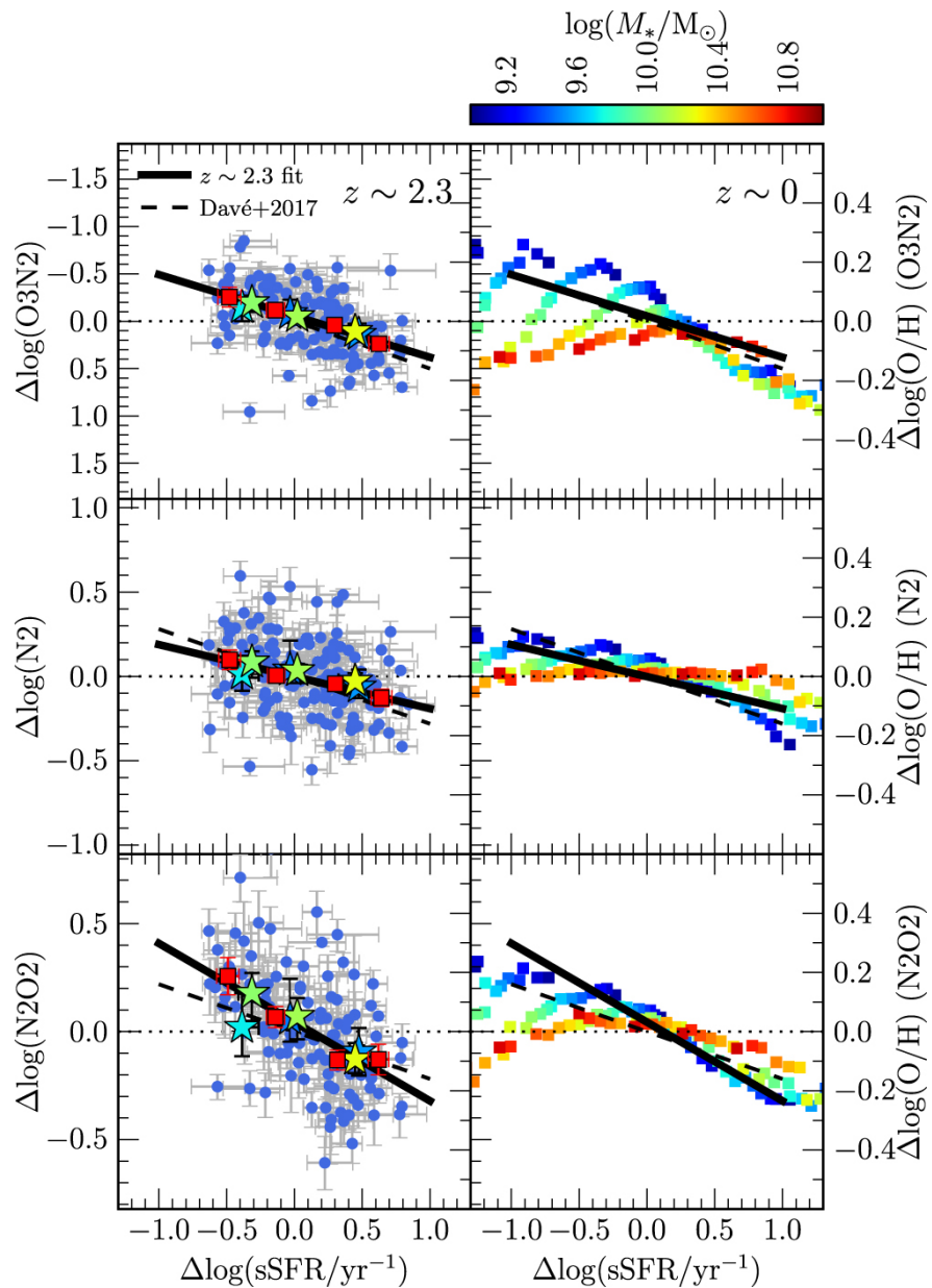
Figure 3. from The MOSDEF Survey: A Stellar Mass–SFR–Metallicity Relation Exists at z \sim 2.3 null 2018 APJ 858 99 doi:10.3847/1538-4357/aabcbdb https://dx.doi.org/10.3847/1538-4357/aabcbdb © 2018. The American Astronomical Society. All rights reserved.
