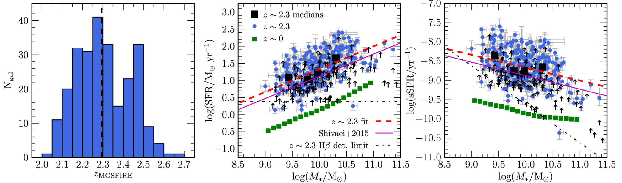
Figure 1. from The MOSDEF Survey: A Stellar Mass–SFR–Metallicity Relation Exists at z \sim 2.3 null 2018 APJ 858 99 doi:10.3847/1538-4357/aabcbdb https://dx.doi.org/10.3847/1538-4357/aabcbdb © 2018. The American Astronomical Society. All rights reserved.
