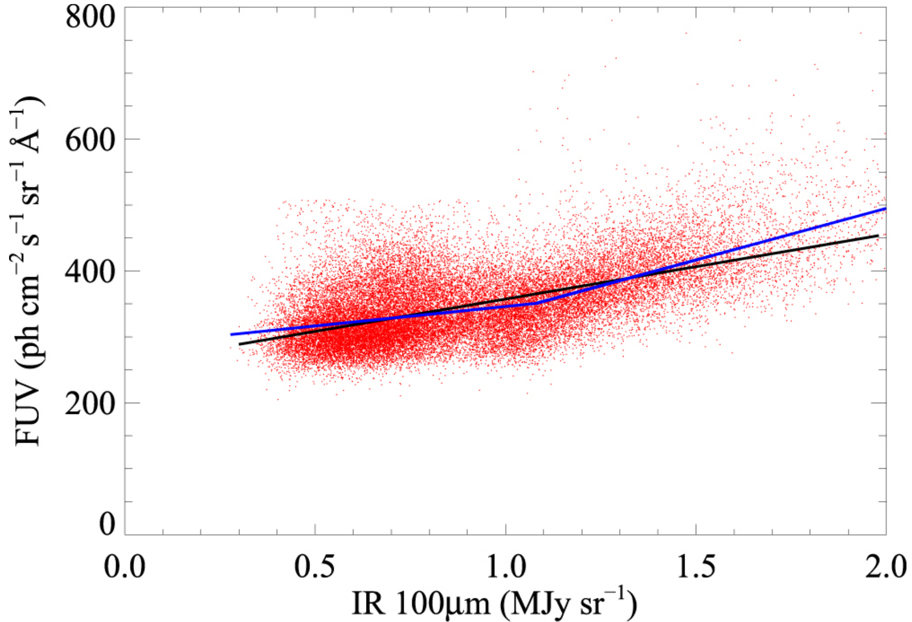
Figure 5. from The Diffuse Radiation Field at High Galactic Latitudes null 2018 APJ 858 101 doi:10.3847/1538-4357/aabcb9 https://dx.doi.org/10.3847/1538-4357/aabcb9 © 2018. The American Astronomical Society. All rights reserved.
