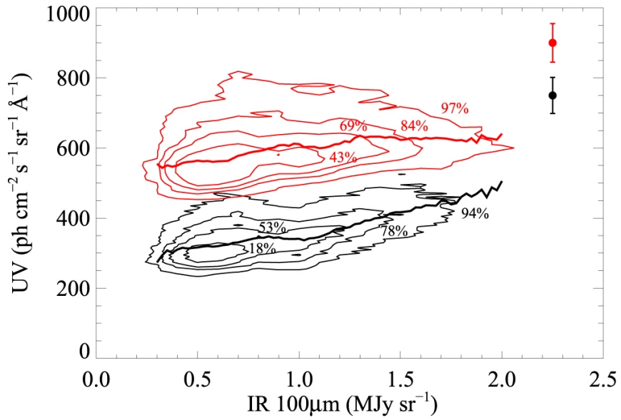
Figure 4. from The Diffuse Radiation Field at High Galactic Latitudes null 2018 APJ 858 101 doi:10.3847/1538-4357/aabcb9 https://dx.doi.org/10.3847/1538-4357/aabcb9 © 2018. The American Astronomical Society. All rights reserved.
