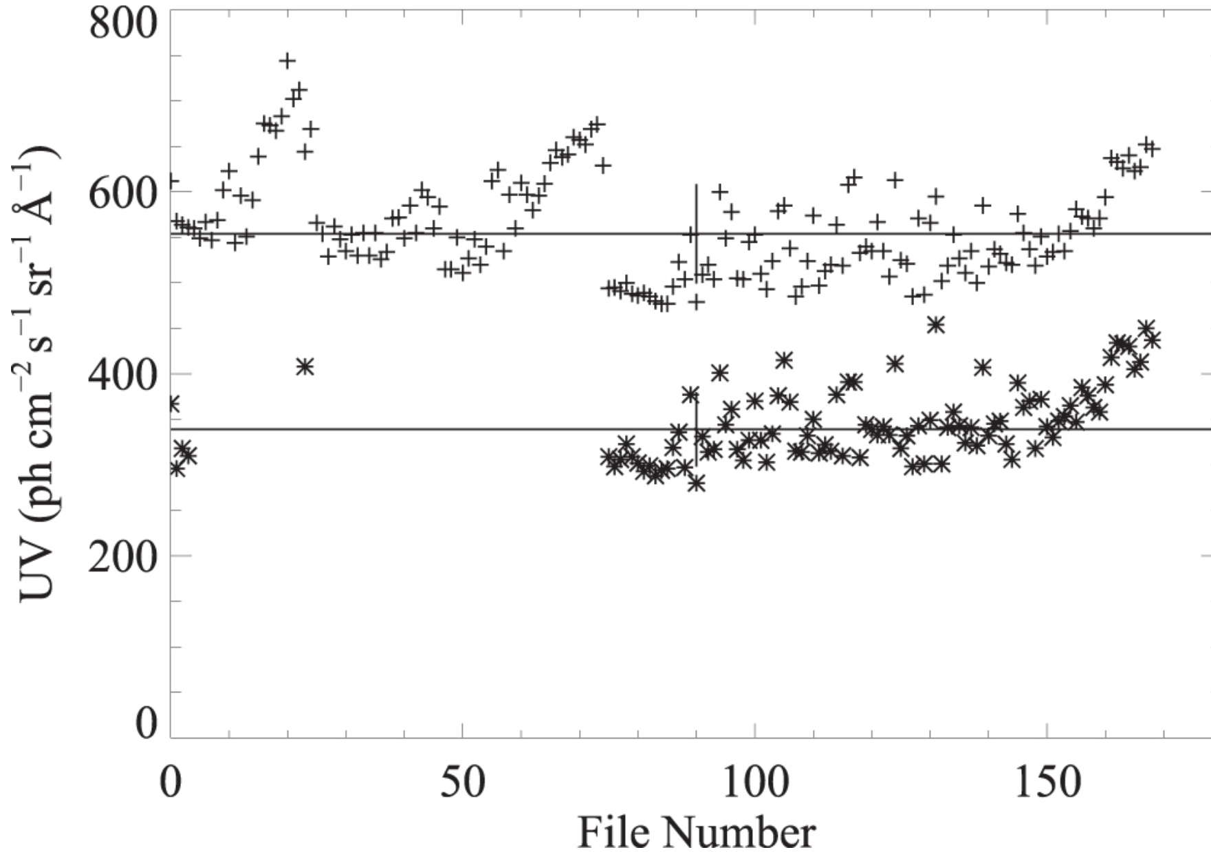
Figure 3. from The Diffuse Radiation Field at High Galactic Latitudes null 2018 APJ 858 101 doi:10.3847/1538-4357/aabcb9 https://dx.doi.org/10.3847/1538-4357/aabcb9 © 2018. The American Astronomical Society. All rights reserved.
