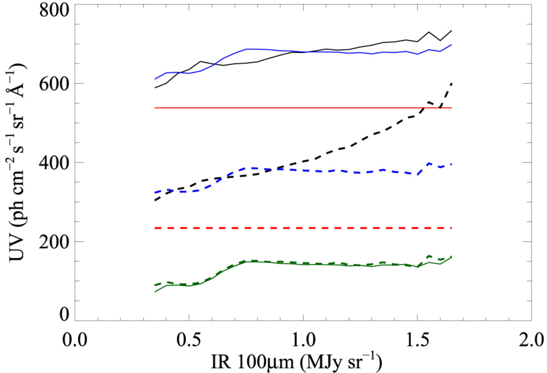
Figure 13. from The Diffuse Radiation Field at High Galactic Latitudes null 2018 APJ 858 101 doi:10.3847/1538-4357/aabcb9 https://dx.doi.org/10.3847/1538-4357/aabcb9 © 2018. The American Astronomical Society. All rights reserved.
