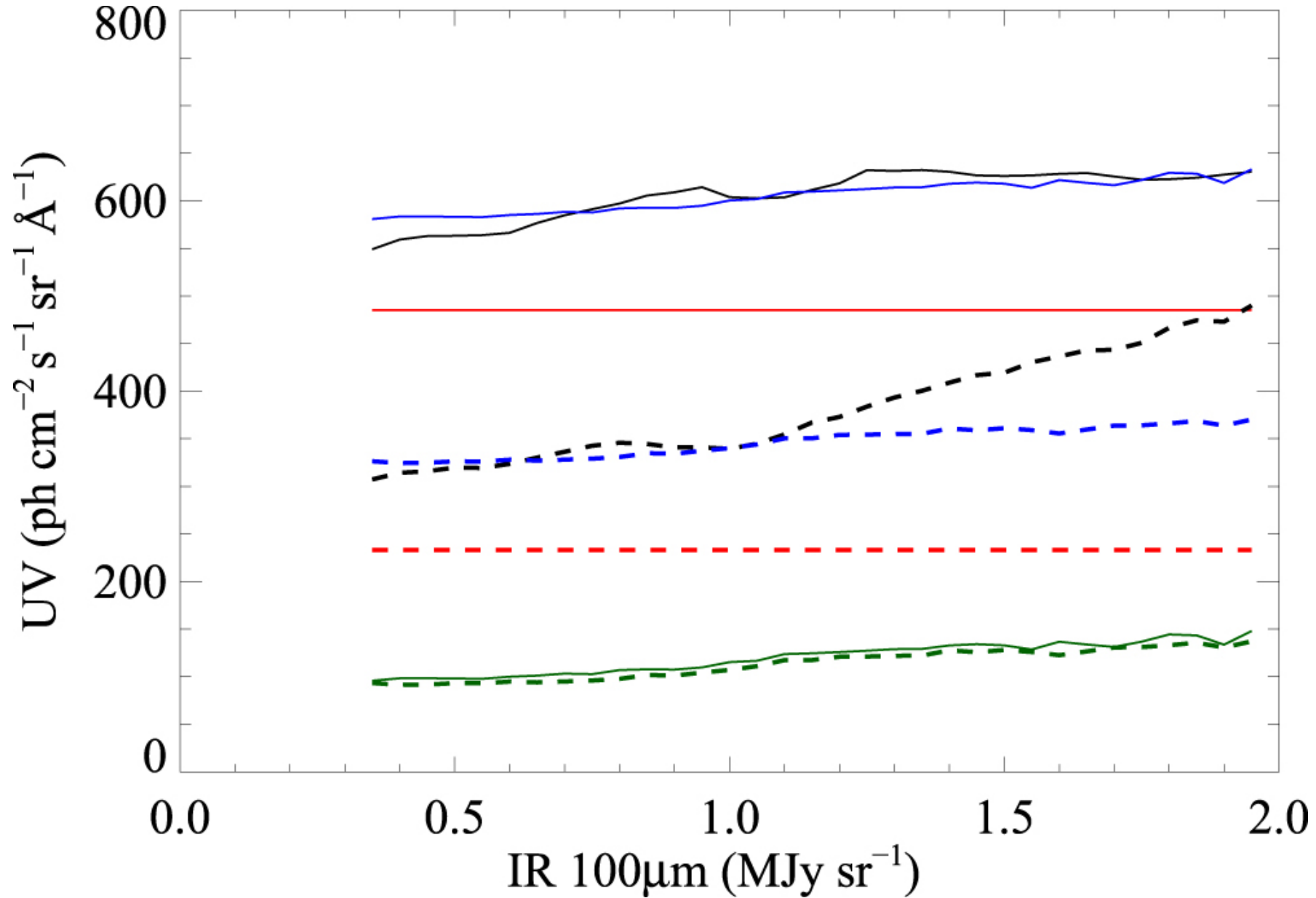
Figure 12. from The Diffuse Radiation Field at High Galactic Latitudes null 2018 APJ 858 101 doi:10.3847/1538-4357/aabcb9 https://dx.doi.org/10.3847/1538-4357/aabcb9 © 2018. The American Astronomical Society. All rights reserved.
