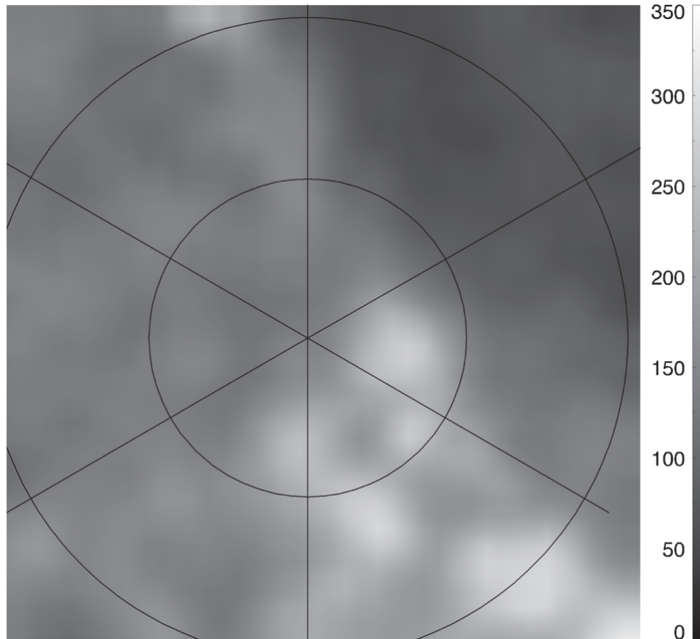
Figure 10. from The Diffuse Radiation Field at High Galactic Latitudes null 2018 APJ 858 101 doi:10.3847/1538-4357/aabcb9 https://dx.doi.org/10.3847/1538-4357/aabcb9 © 2018. The American Astronomical Society. All rights reserved.
