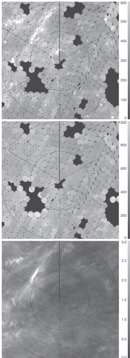
Figure 1. from The Diffuse Radiation Field at High Galactic Latitudes null 2018 APJ 858 101 doi:10.3847/1538-4357/aabcb9 https://dx.doi.org/10.3847/1538-4357/aabcb9 © 2018. The American Astronomical Society. All rights reserved.
