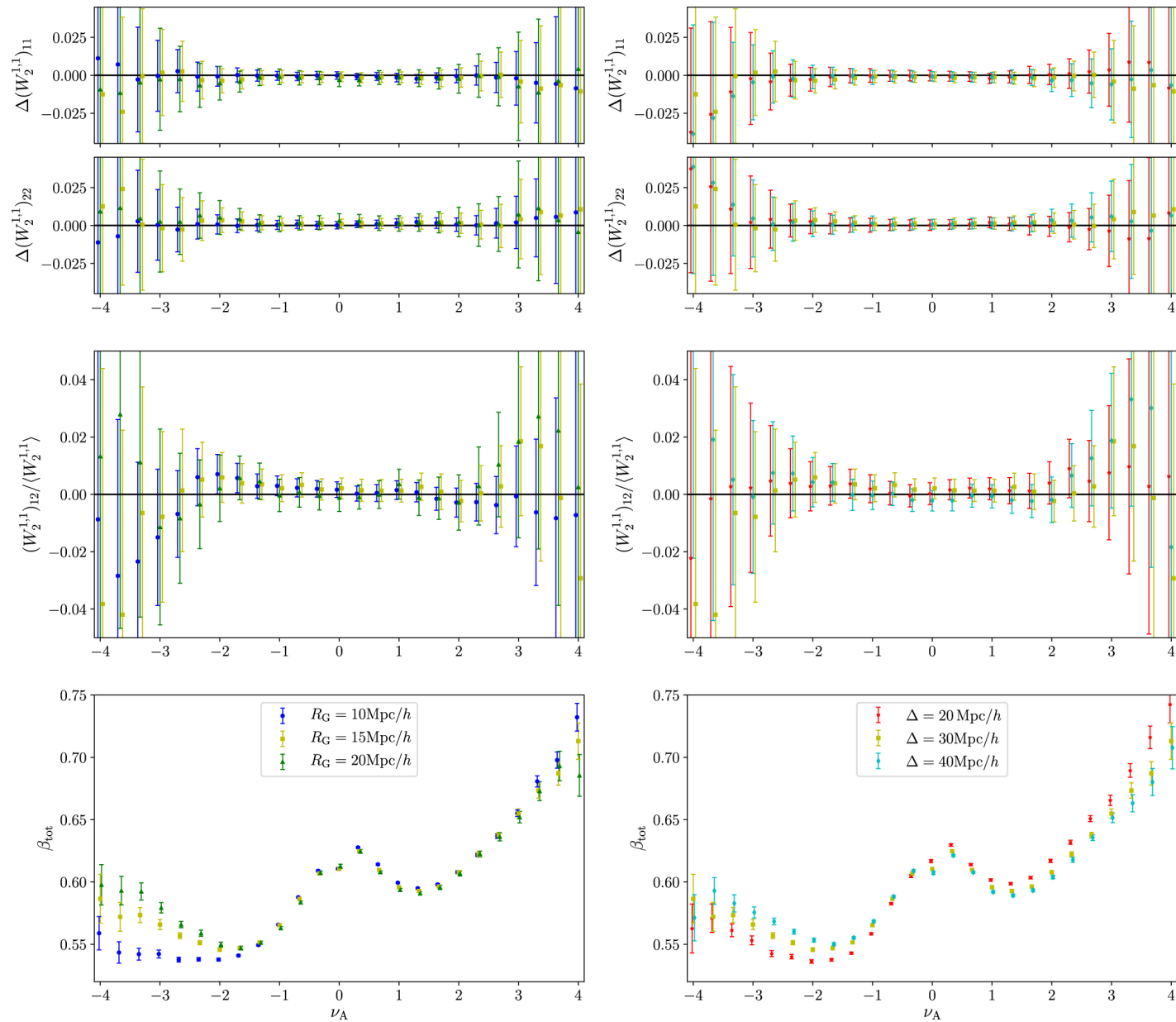
Figure 9. from Minkowski Tensors in Two Dimensions: Probing the Morphology and Isotropy of the Matter and Galaxy Density Fields null 2018 APJ 858 87 doi:10.3847/1538-4357/aabb53 https://dx.doi.org/10.3847/1538-4357/aabb53 © 2018. The American Astronomical Society. All rights reserved.
