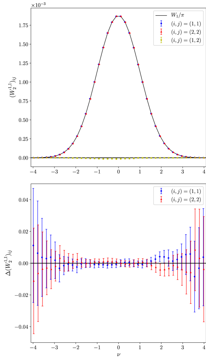
Figure 7. from Minkowski Tensors in Two Dimensions: Probing the Morphology and Isotropy of the Matter and Galaxy Density Fields null 2018 APJ 858 87 doi:10.3847/1538-4357/aabb53 https://dx.doi.org/10.3847/1538-4357/aabb53 © 2018. The American Astronomical Society. All rights reserved.
