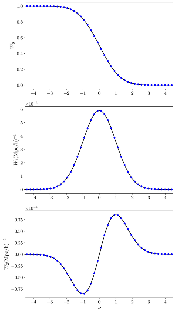
Figure 6. from Minkowski Tensors in Two Dimensions: Probing the Morphology and Isotropy of the Matter and Galaxy Density Fields null 2018 APJ 858 87 doi:10.3847/1538-4357/aabb53 https://dx.doi.org/10.3847/1538-4357/aabb53 © 2018. The American Astronomical Society. All rights reserved.
