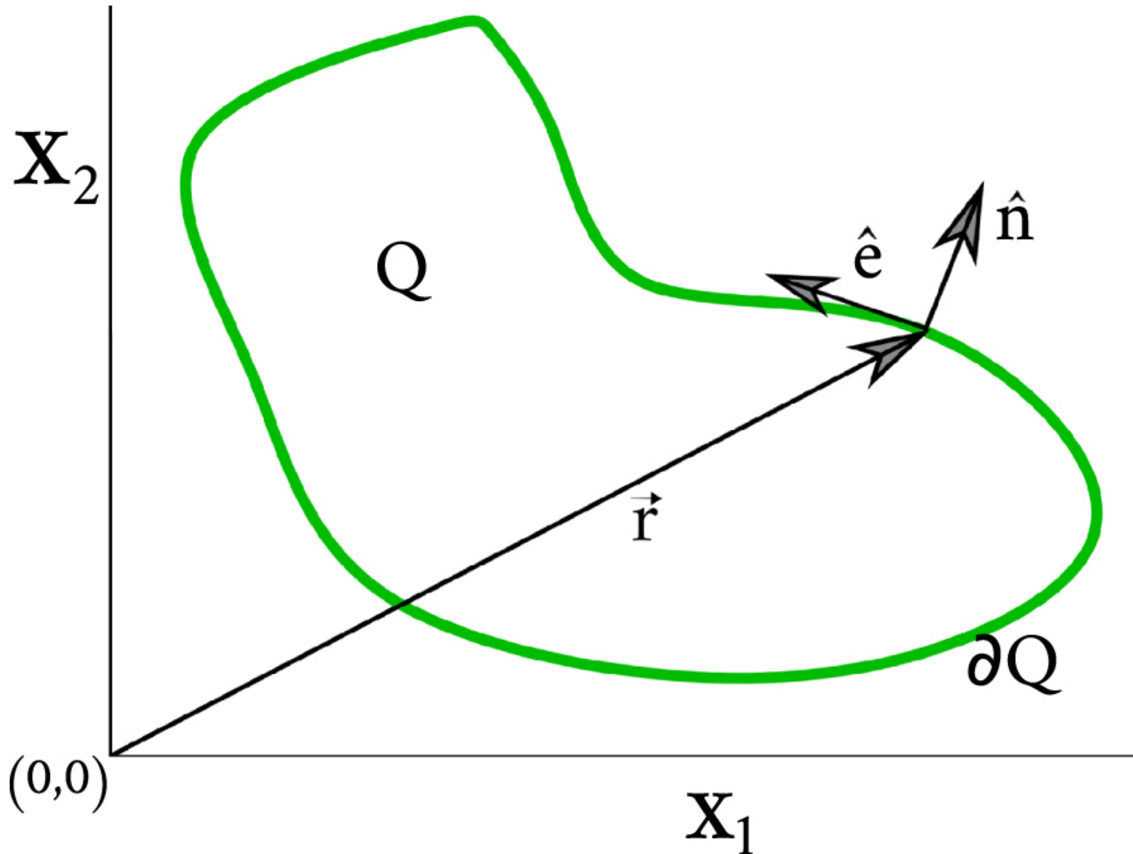
Figure 4. from Minkowski Tensors in Two Dimensions: Probing the Morphology and Isotropy of the Matter and Galaxy Density Fields null 2018 APJ 858 87 doi:10.3847/1538-4357/aabb53 https://dx.doi.org/10.3847/1538-4357/aabb53 © 2018. The American Astronomical Society. All rights reserved.
