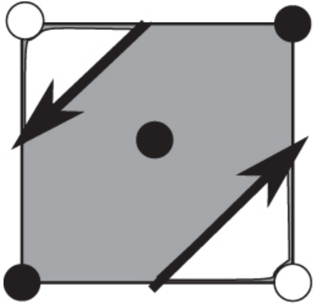
Figure 2. from Minkowski Tensors in Two Dimensions: Probing the Morphology and Isotropy of the Matter and Galaxy Density Fields null 2018 APJ 858 87 doi:10.3847/1538-4357/aabb53 https://dx.doi.org/10.3847/1538-4357/aabb53 © 2018. The American Astronomical Society. All rights reserved.
