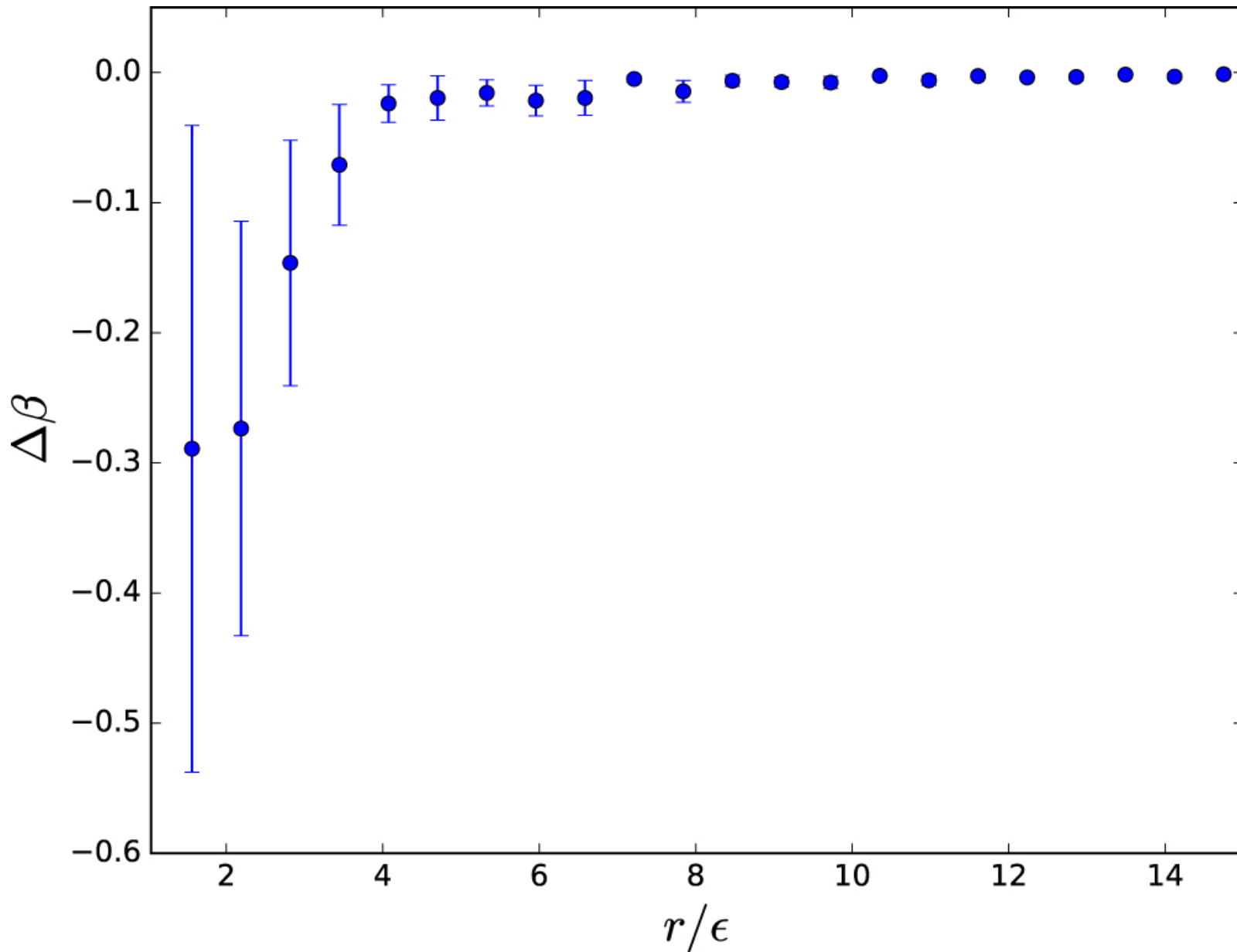
Figure 15. from Minkowski Tensors in Two Dimensions: Probing the Morphology and Isotropy of the Matter and Galaxy Density Fields null 2018 APJ 858 87 doi:10.3847/1538-4357/aabb53 https://dx.doi.org/10.3847/1538-4357/aabb53 © 2018. The American Astronomical Society. All rights reserved.
