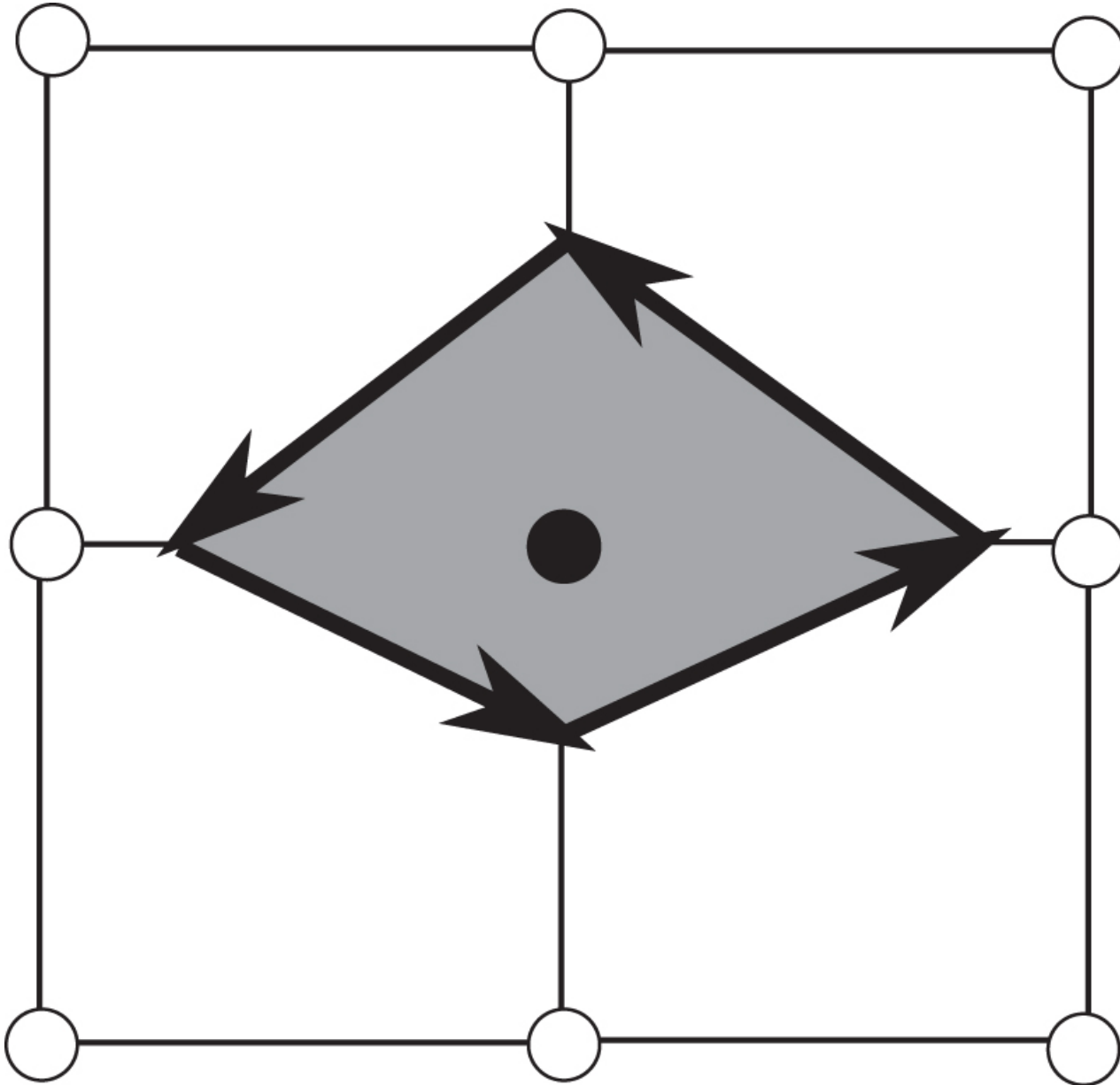
Figure 14. from Minkowski Tensors in Two Dimensions: Probing the Morphology and Isotropy of the Matter and Galaxy Density Fields null 2018 APJ 858 87 doi:10.3847/1538-4357/aabb53 https://dx.doi.org/10.3847/1538-4357/aabb53 © 2018. The American Astronomical Society. All rights reserved.
