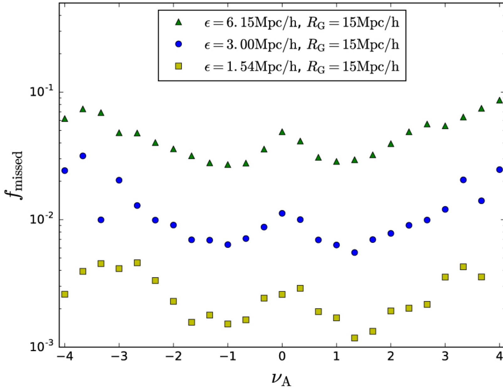
Figure 13. from Minkowski Tensors in Two Dimensions: Probing the Morphology and Isotropy of the Matter and Galaxy Density Fields null 2018 APJ 858 87 doi:10.3847/1538-4357/aabb53 https://dx.doi.org/10.3847/1538-4357/aabb53 © 2018. The American Astronomical Society. All rights reserved.
