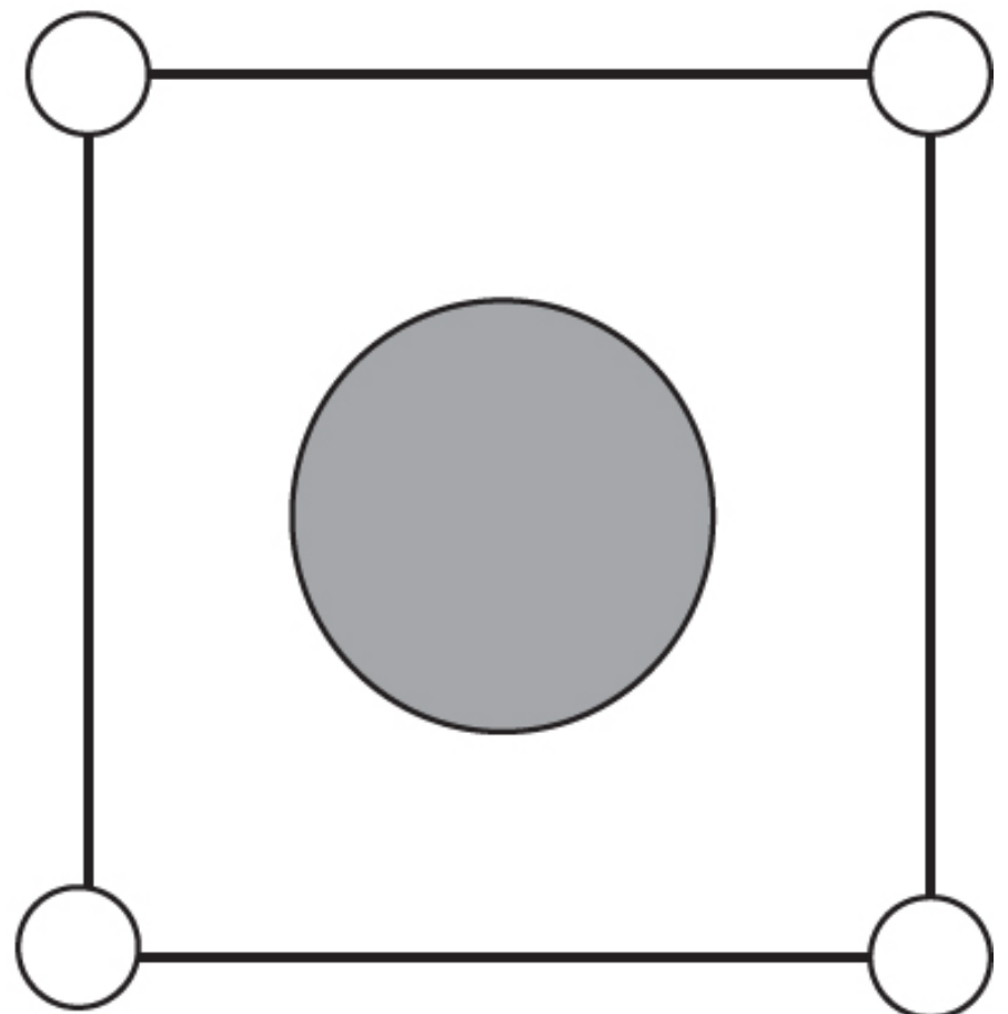
Figure 12. from Minkowski Tensors in Two Dimensions: Probing the Morphology and Isotropy of the Matter and Galaxy Density Fields null 2018 APJ 858 87 doi:10.3847/1538-4357/aabb53 https://dx.doi.org/10.3847/1538-4357/aabb53 © 2018. The American Astronomical Society. All rights reserved.
