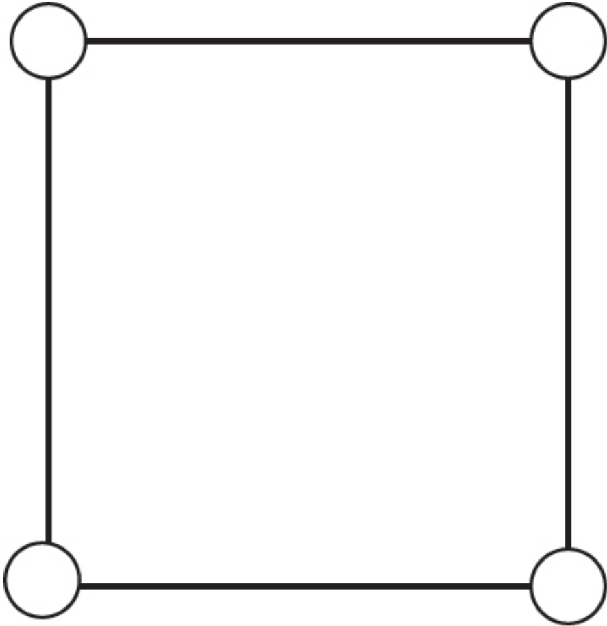
Figure 12. from Minkowski Tensors in Two Dimensions: Probing the Morphology and Isotropy of the Matter and Galaxy Density Fields null 2018 APJ 858 87 doi:10.3847/1538-4357/aabb53 https://dx.doi.org/10.3847/1538-4357/aabb53 © 2018. The American Astronomical Society. All rights reserved.
