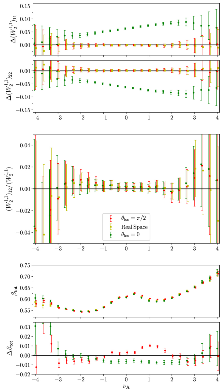
Figure 11. from Minkowski Tensors in Two Dimensions: Probing the Morphology and Isotropy of the Matter and Galaxy Density Fields null 2018 APJ 858 87 doi:10.3847/1538-4357/aabb53 https://dx.doi.org/10.3847/1538-4357/aabb53
