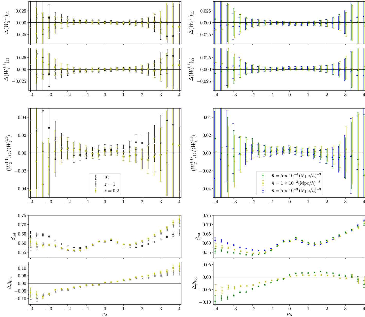
Figure 10. from Minkowski Tensors in Two Dimensions: Probing the Morphology and Isotropy of the Matter and Galaxy Density Fields null 2018 APJ 858 87 doi:10.3847/1538-4357/aabb53 https://dx.doi.org/10.3847/1538-4357/aabb53
