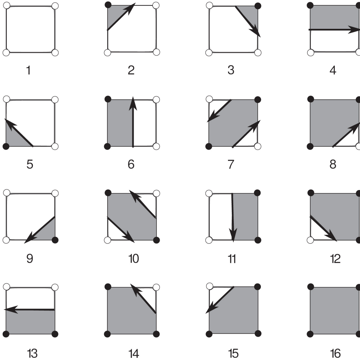
Figure 1. from Minkowski Tensors in Two Dimensions: Probing the Morphology and Isotropy of the Matter and Galaxy Density Fields null 2018 APJ 858 87 doi:10.3847/1538-4357/aabb53 https://dx.doi.org/10.3847/1538-4357/aabb53
