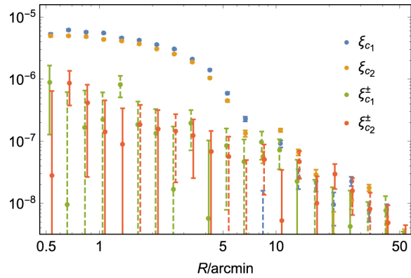
Figure 6. from Removing the Impact of Correlated PSF Uncertainties in Weak Lensing null 2018 APJ 858 122 doi:10.3847/1538-4357/aabb50 https://dx.doi.org/10.3847/1538-4357/aabb50 © 2018. The American Astronomical Society. All rights reserved.
