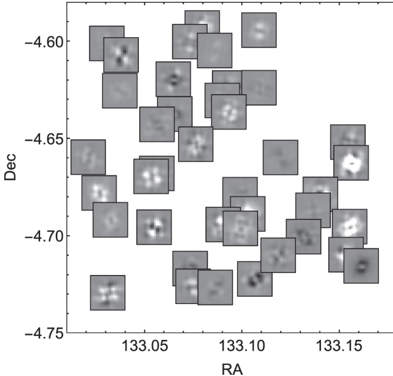
Figure 1. from Removing the Impact of Correlated PSF Uncertainties in Weak Lensing null 2018 APJ 858 122 doi:10.3847/1538-4357/aabb50 https://dx.doi.org/10.3847/1538-4357/aabb50 © 2018. The American Astronomical Society. All rights reserved.
